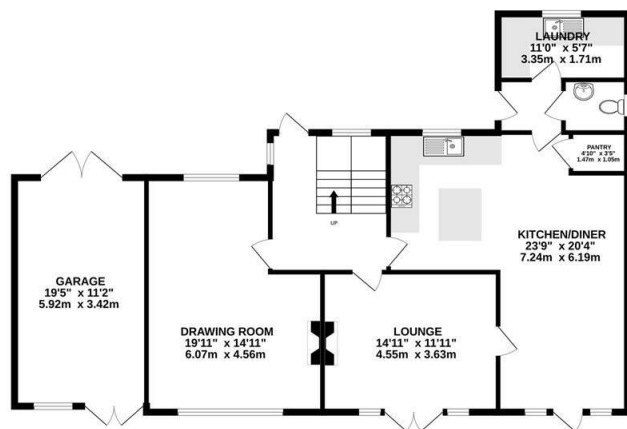
GROUND FLOOR 1251 sq.ft. (116.2 sq.m.) approx.
